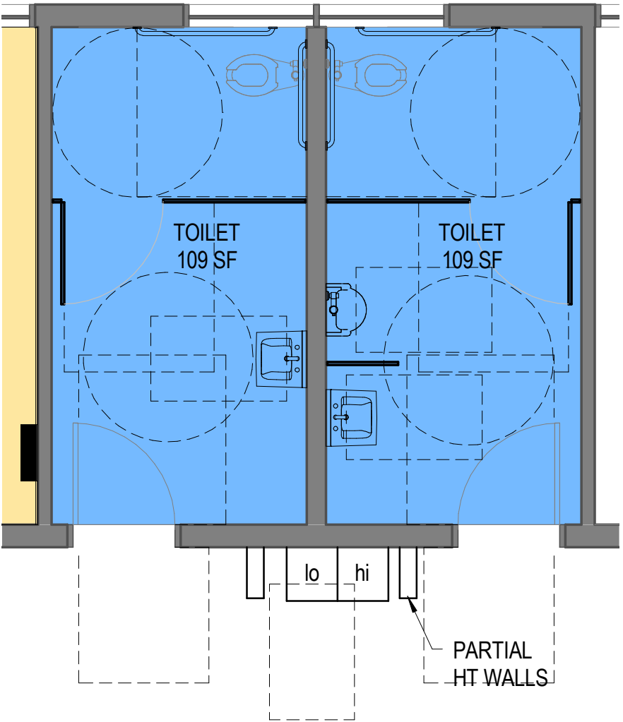
2 FLOOR PLAN - PROPOSED TOILETS 1/4" = 1'-0"
