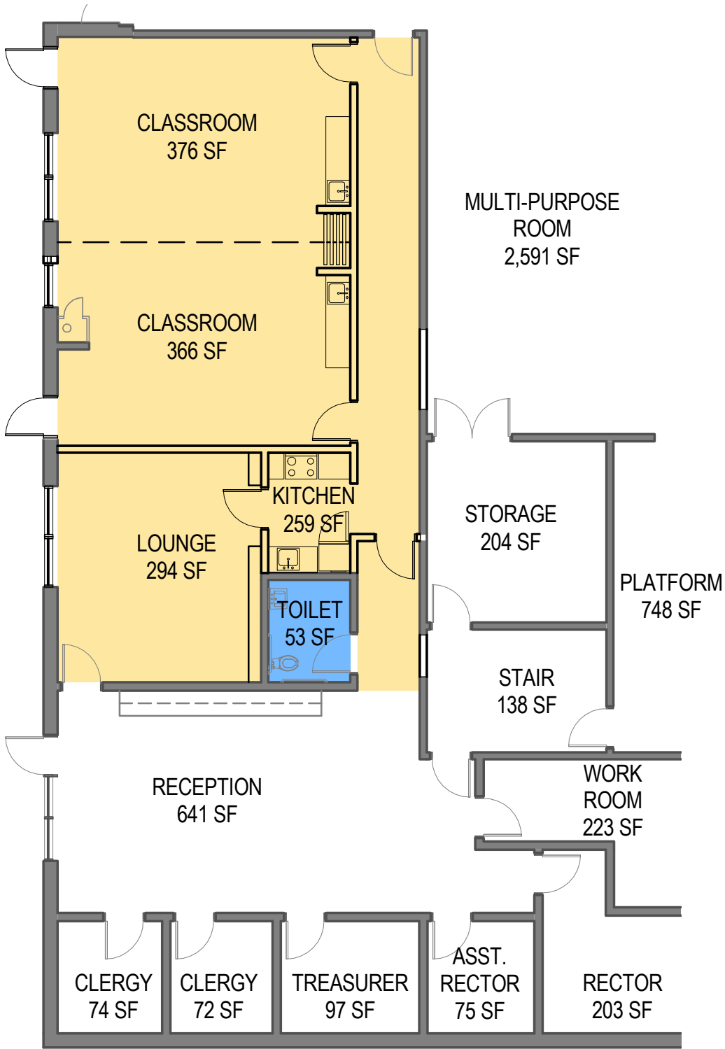
2 ENLARGED MP PLAN 3/32" = 1'-0"
